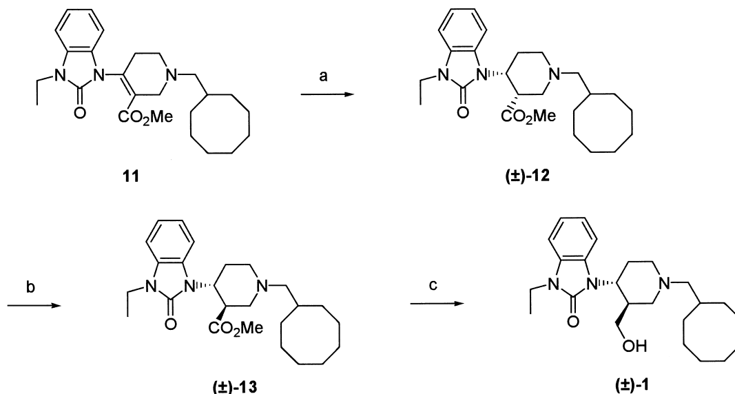
Scheme 4. (a) H 2 , Pd/C 10%, MeOH, 50%. (b) MeONa, MeOH, rt, 92%. (c) LiAlH 4 , Et 2 O, 0°C, 80%.
