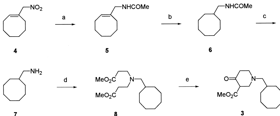
Scheme 2. (a) i: \text{LiAlH}_4 , EtO, 0^\circ\text{C} ; ii: \text{Et}_3\text{N} , \text{Ac}_2\text{O} , \text{CH}_2\text{Cl}_2 , 0^\circ\text{C} 78% over two steps. (b) \text{H}_2 , Pd/C 10%, EtOH, 96%. (c) HCl, EtOH/ \text{H}_2\text{O} , \Delta , 84%. (d) \text{CH}_2=\text{CH}-\text{CO}_2\text{OMe} , MeOH rt, 72%. (e) t -BuOK, toluene, rt, 78%.
