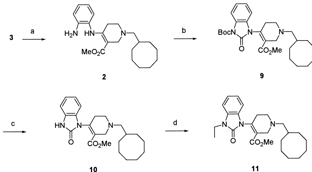
Scheme 3. (a) o -phenylenediamine, AcOH, molecular sieves, benzene, \Delta , 83%. (b) (Boc) 2 O, DMAP, CH 2 Cl 2 , 0°C, 89%. (c) TFA, CH 2 Cl 2 , rt, 97%. (d) NaH, EtBr, DMF, rt, 75%.
